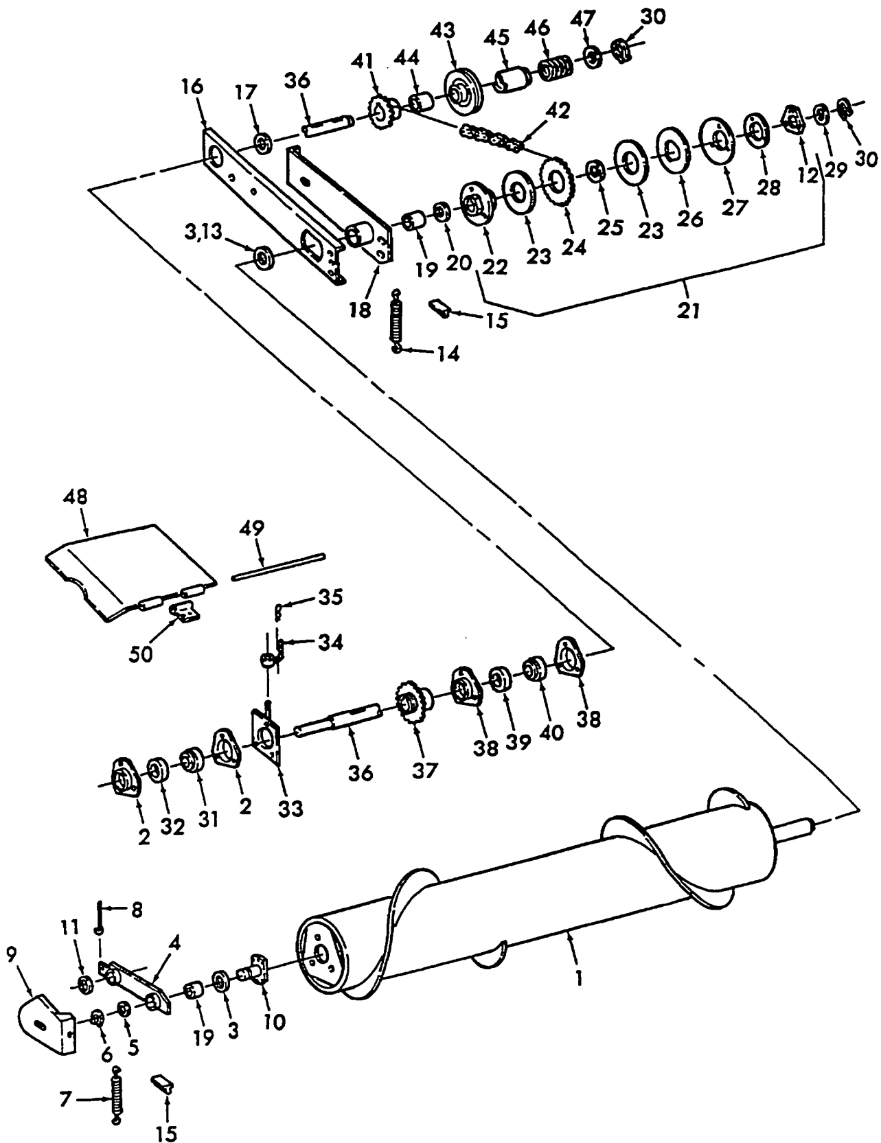
FIG. 2 - AUGER & AUGER DRIVE - 890W
