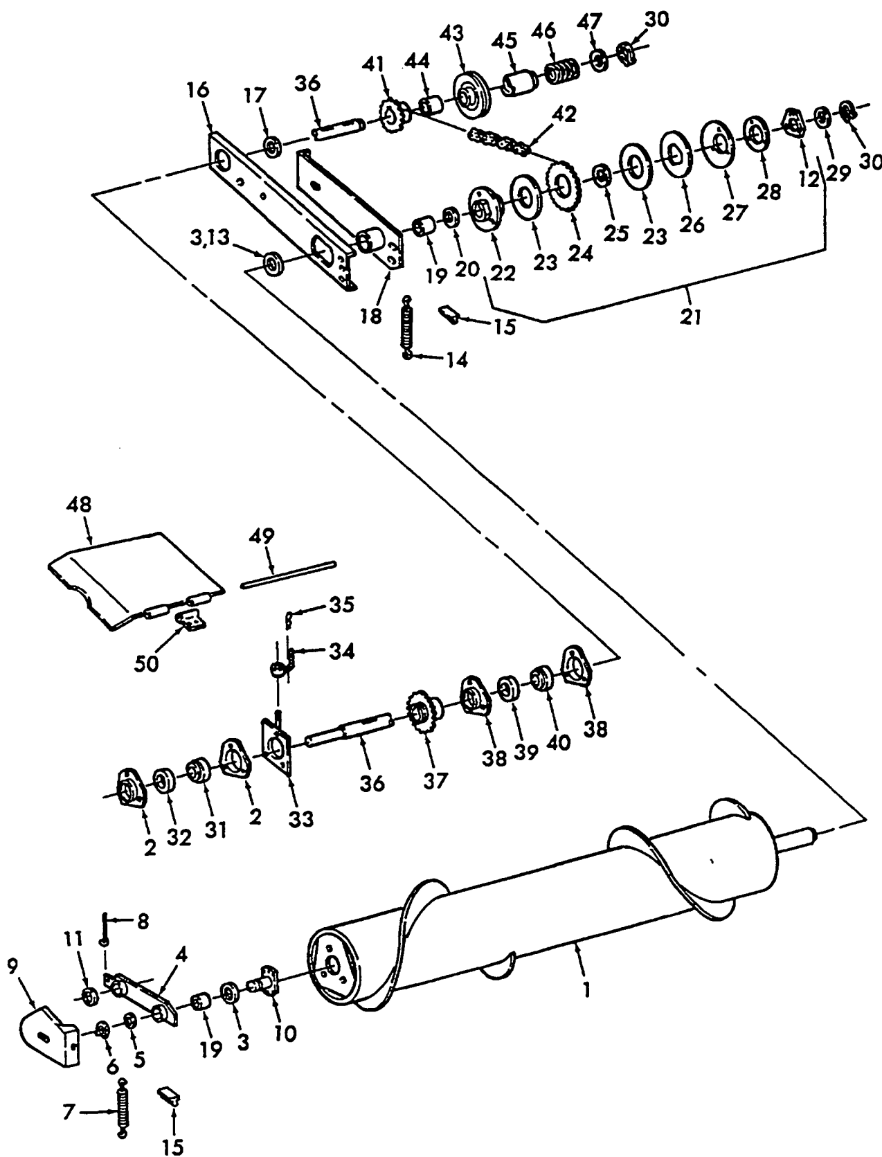
FIG. 2 - AUGER &amp; AUGER DRIVE - 890W
