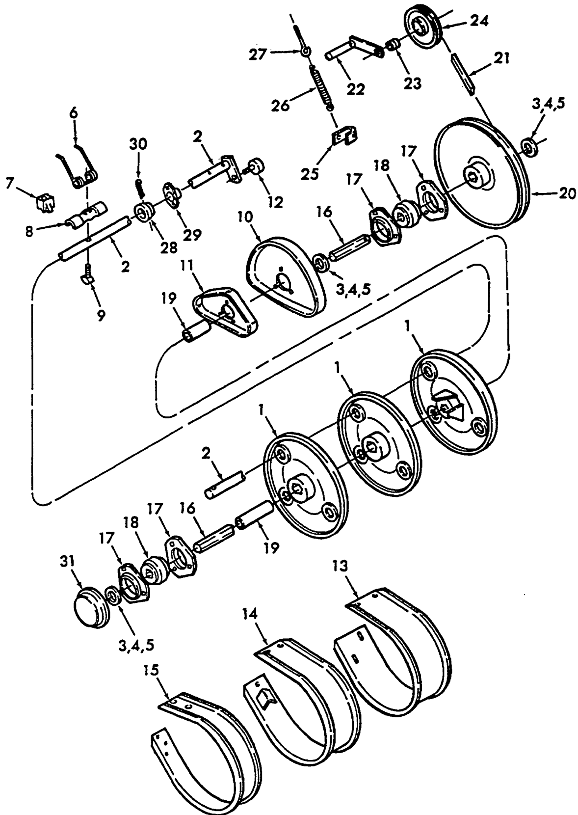
FIG. 3 - PICK-UP & PICK-UP DRIVE - 890W
