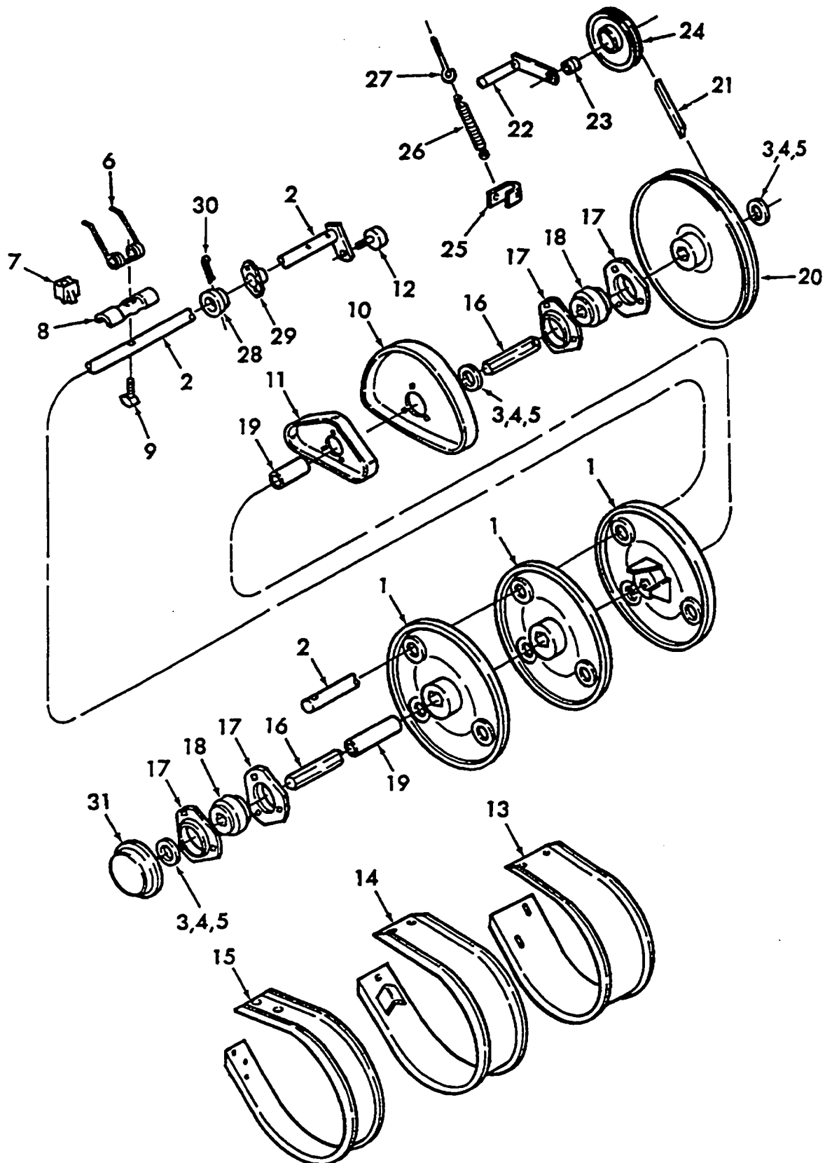
FIG. 3 - PICK-UP &amp; PICK-UP DRIVE - 890W
